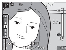
Peaking-taso
