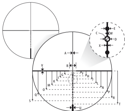
BDC 800 reticle
